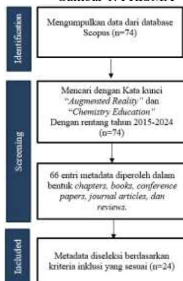
Gambar 1. PRISMA
