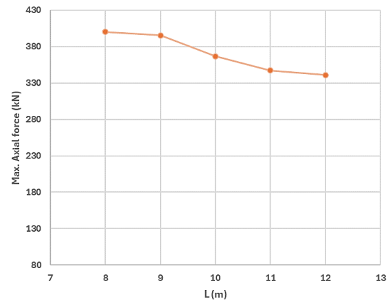
Figure 7. Effect of nail bar length (L) to axial force
