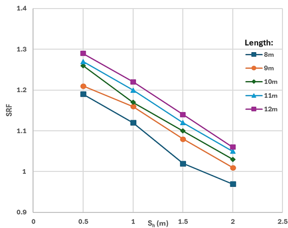
Figure 9. Effect of nail bar horizontal distance ( S_h ) to SRF
