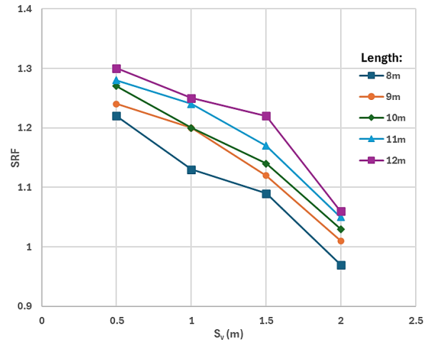
Figure 12. Effect of nail bar vertical distance ( S_v ) to SRF
