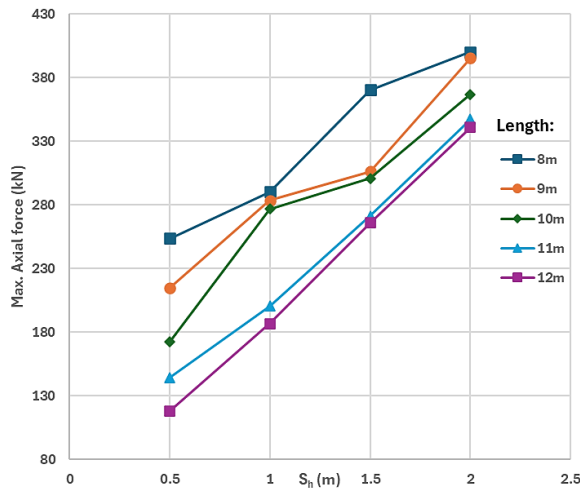
Figure 11. Effect of nail bar horizontal distance ( S_h ) to axial force
