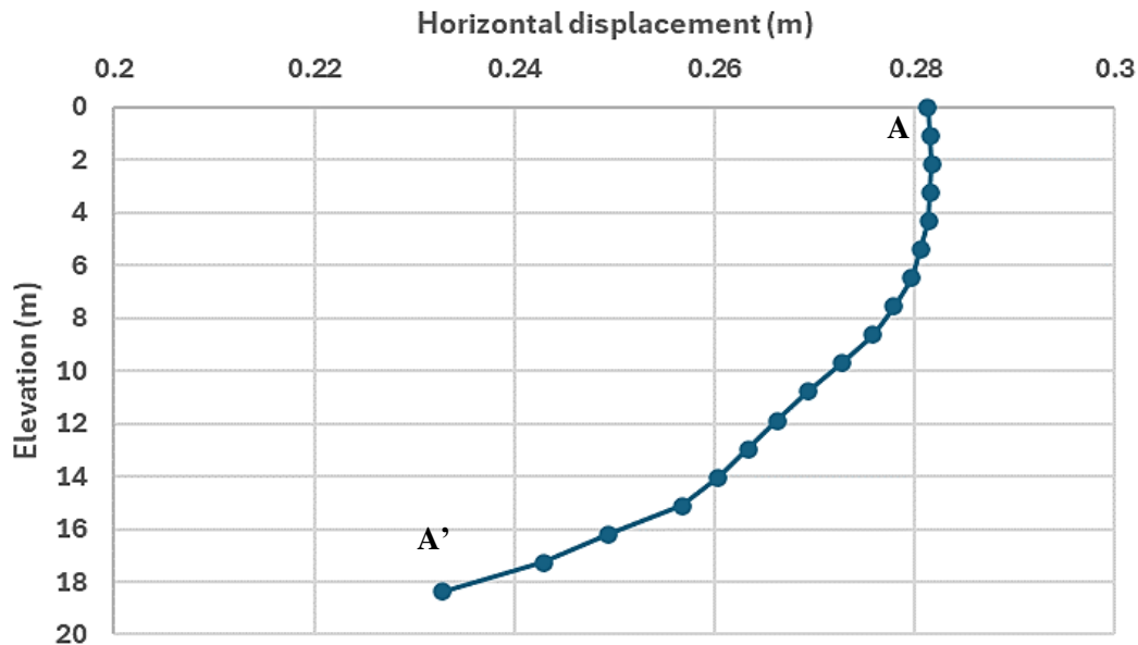
Figure 16. Effect of elevation to displacement
