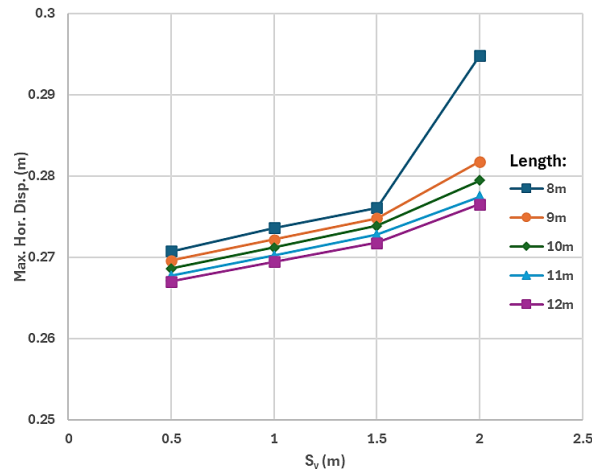
Figure 13. Effect of nail bar vertical distance ( S_v ) to maximum horizontal displacement
