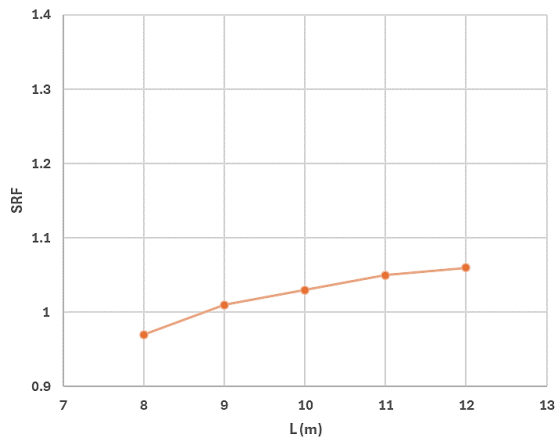
Figure 5. Effect of nail bar length (L) to SRF
