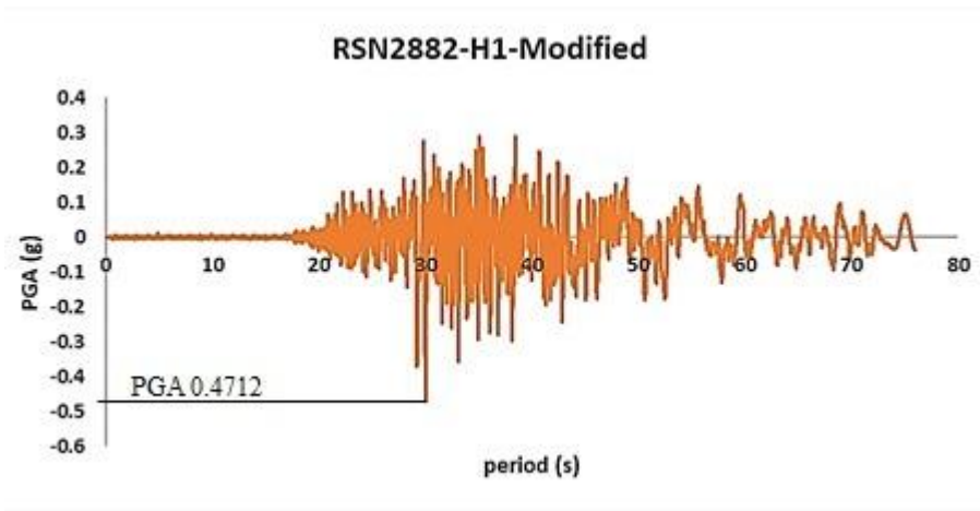
Figure 4. Modified ground motion
