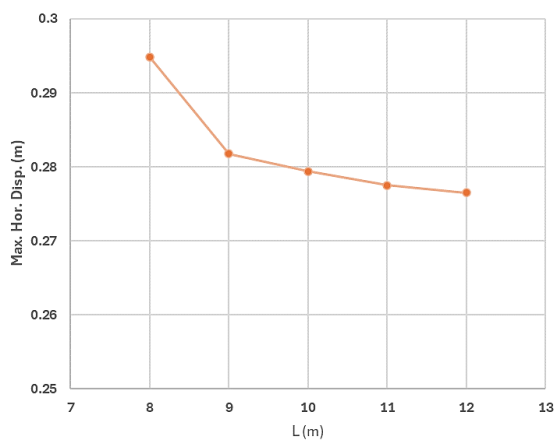
Figure 6. Effect of nail bar length (L) to maximum horizontal displacement
