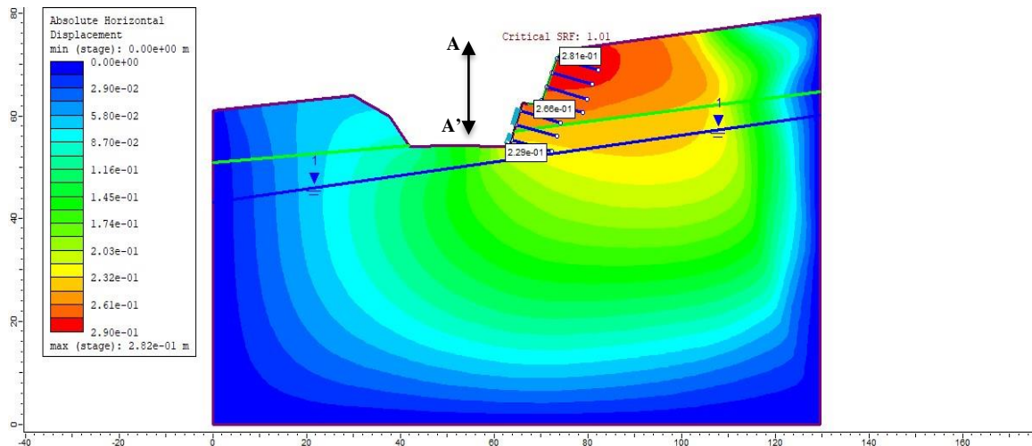
Figure 15. Displacement on pseudo-static condition
