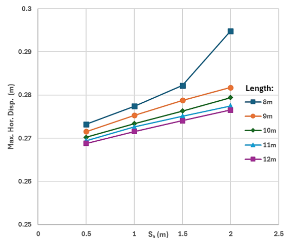
Figure 10. Effect of nail bar horizontal distance ( S_h ) to maximum horizontal displacement
