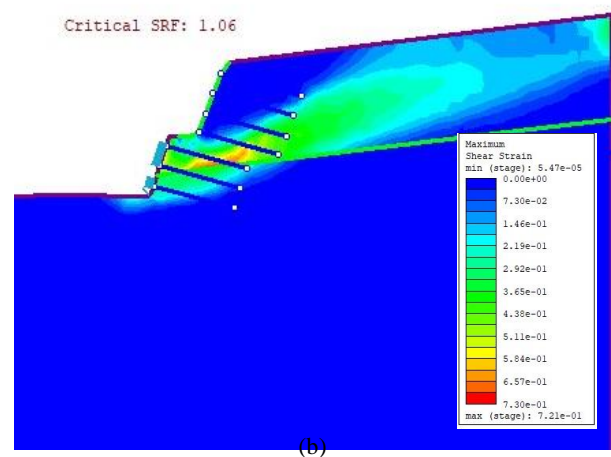
Figure 8. Effect of nail bar length on slip surface (a) L = 8m, (b) L = 12m
