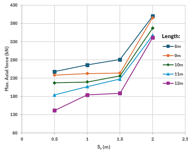
Figure 14. Effect of nail bar vertical distance ( S_v ) to axial force
