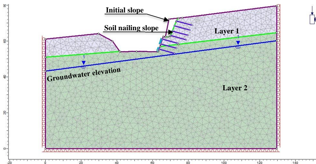
Figure 2. Geometry and meshing of the finite element model
